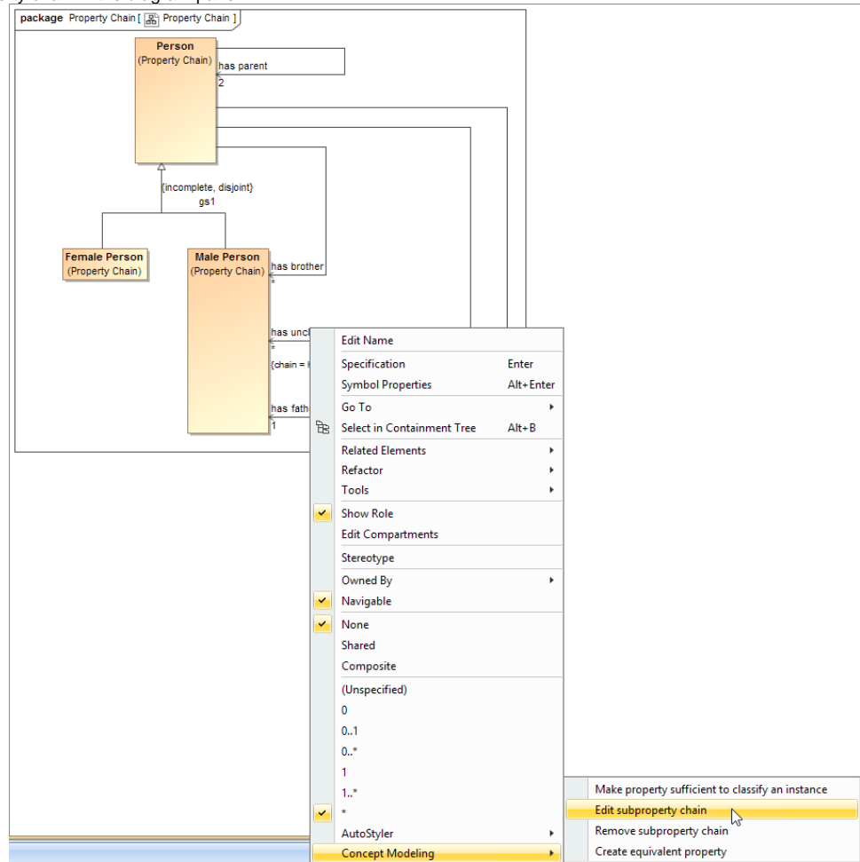
Figure 1: The Edit subproperty chain shortcut menu to edit a property chain.
