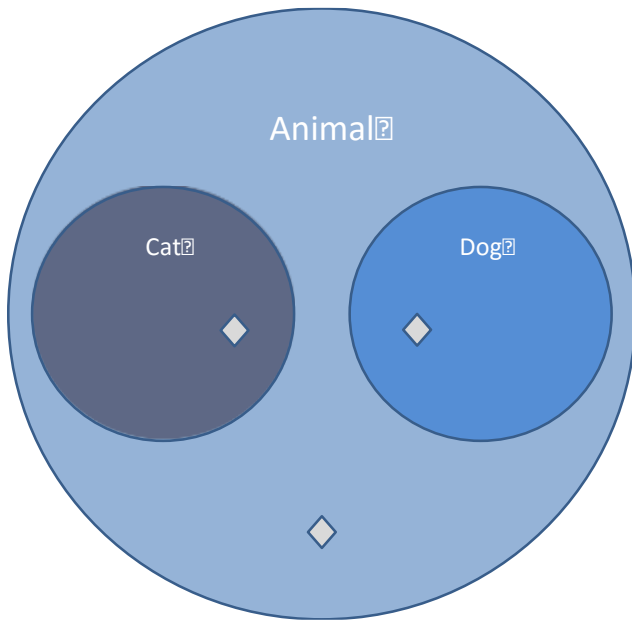
Figure 11 Disjoint instances
