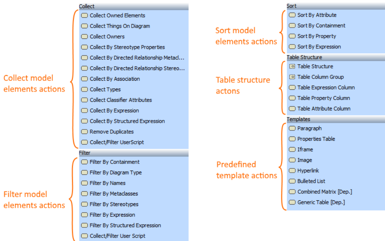
The diagram palette containing predefined actions available in a Viewpoint Method Diagram.
