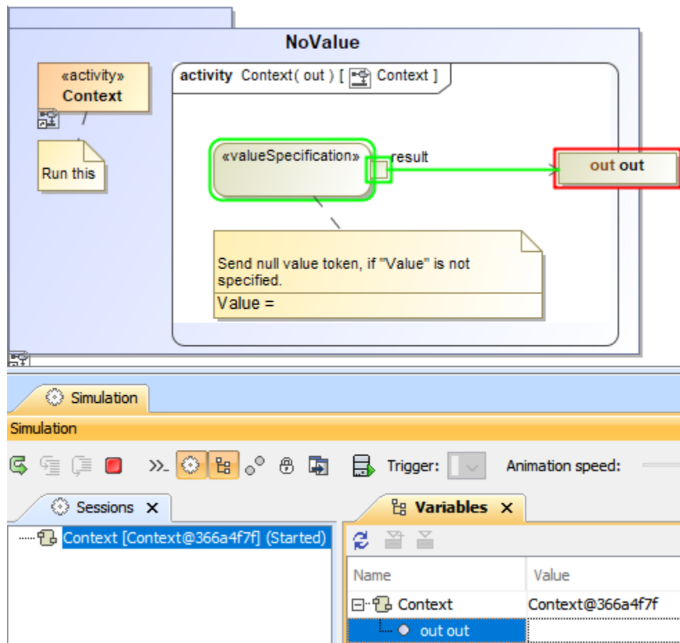
A demo showing the situation when the value of a ValueSpecification Action is unspecified (A null value token is passed.).
