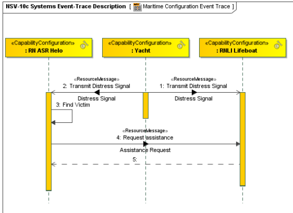
NSV-10c Systems Event-Trace Description
