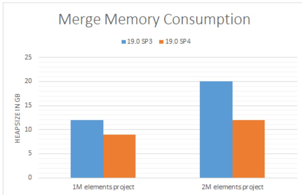
Comparing memory consumption between different versions
