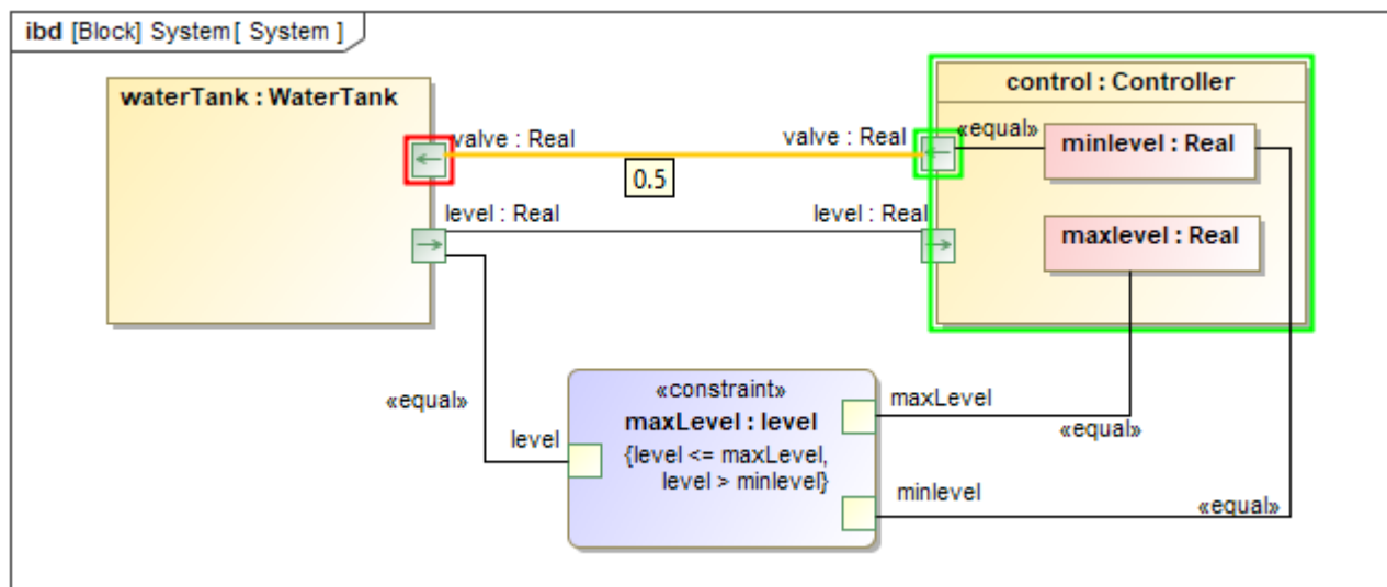
Animation of value propagation in the Internal Block diagram.
