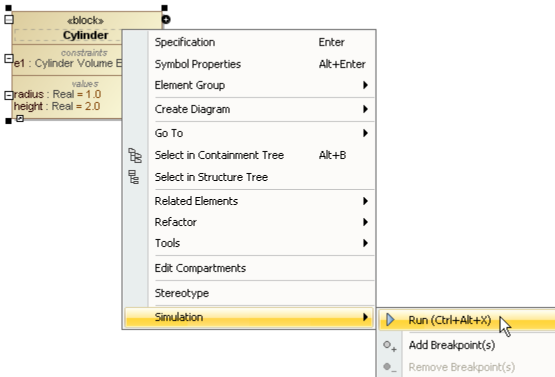
Running a SysML block that has no defined Classifier Behavior.
