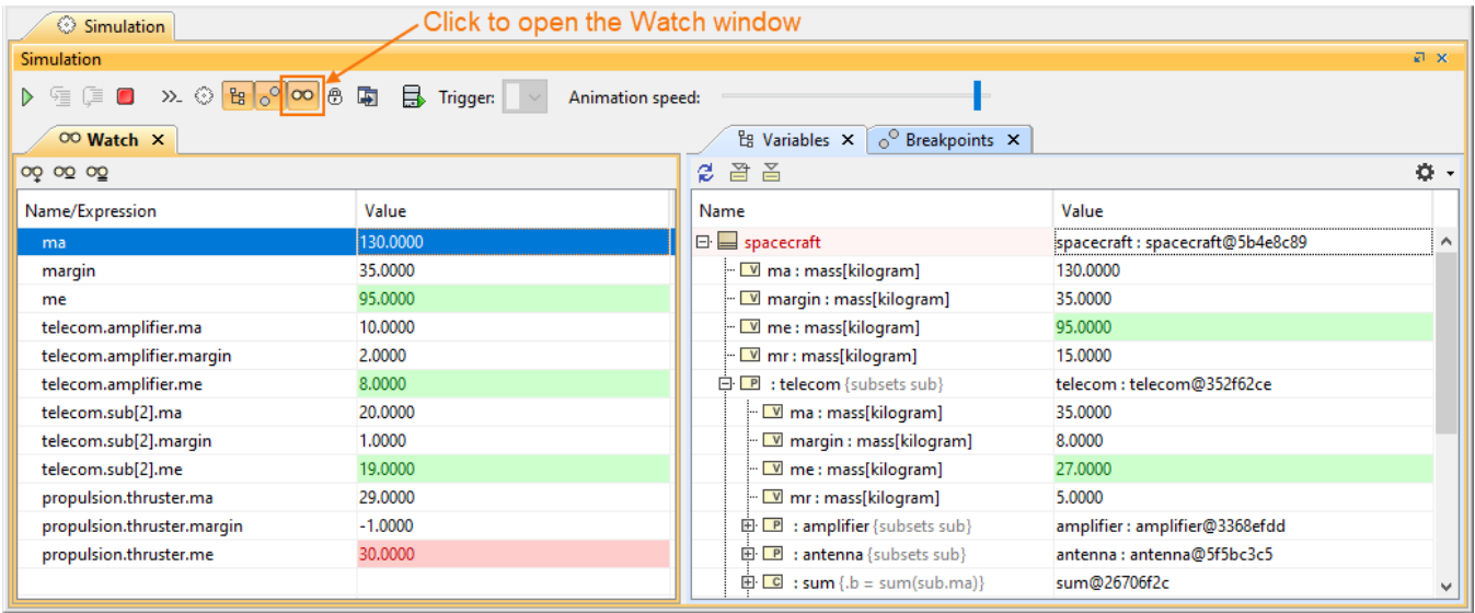
The Watch pane with expressions and their selected runtime values during model simulation.
