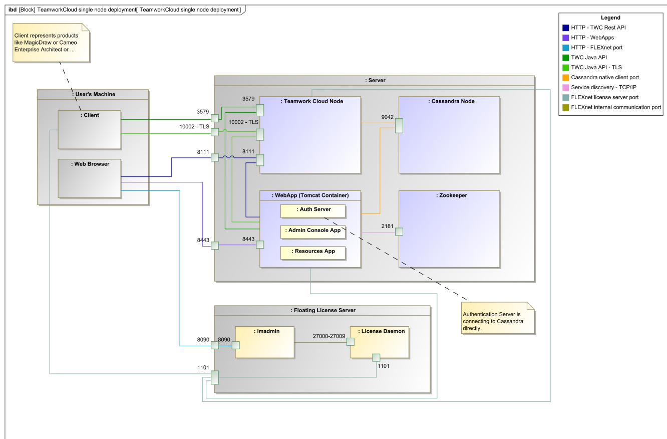
Teamwork Cloud installation and configuration on a single Windows server.
