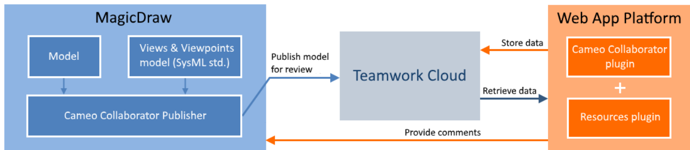
The conceptual schema of Cameo Collaborator for Magic Collaboration Studio.
