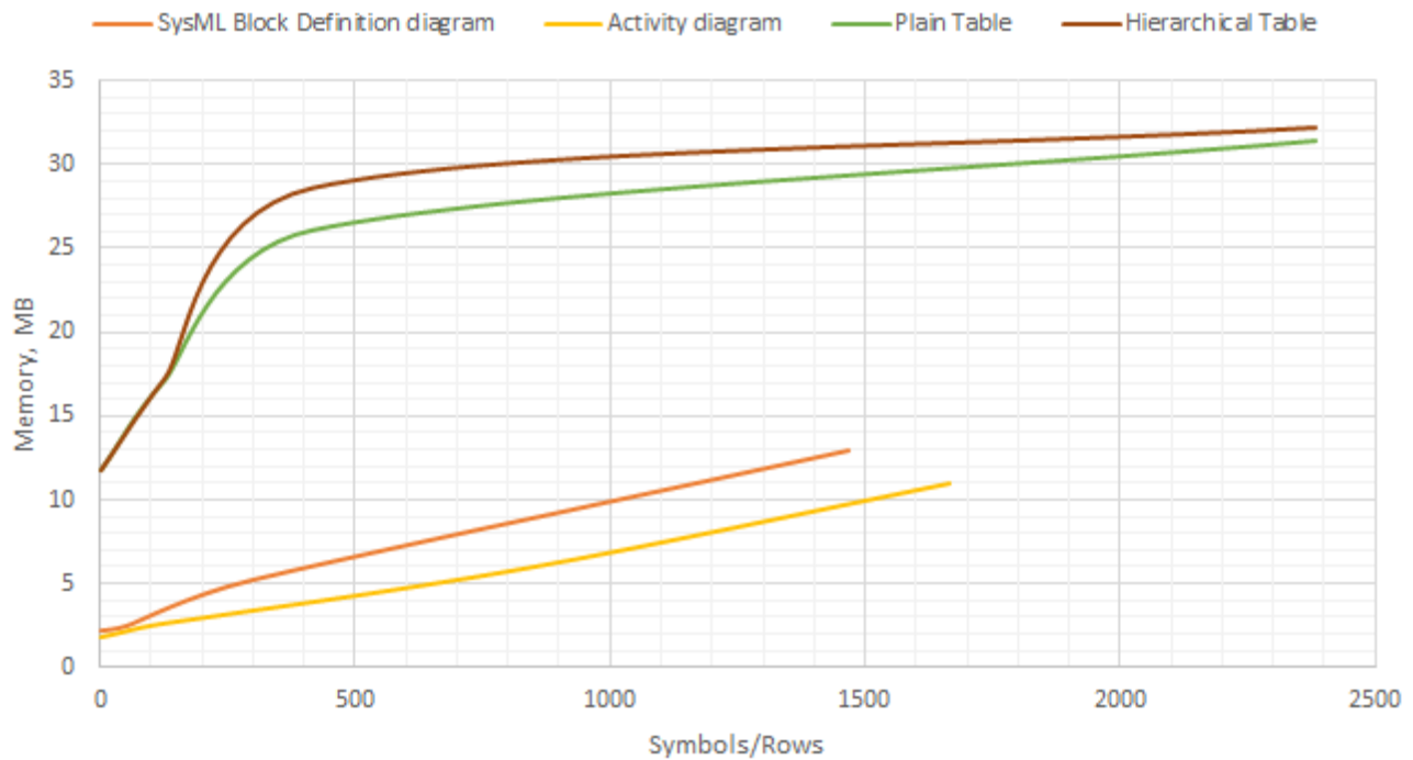
Chart depicting memory consumption by diagram size (symbols/rows displayed in a diagram/table).
