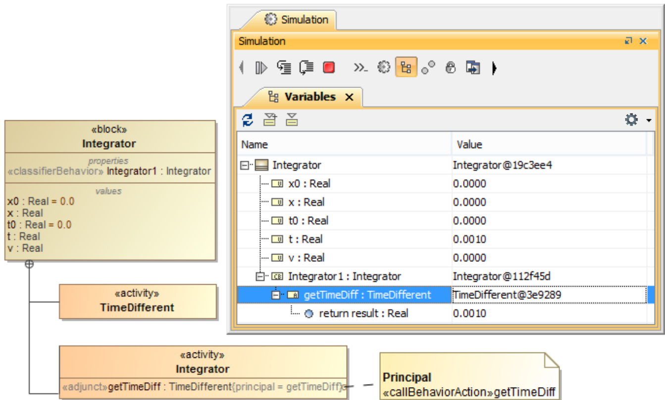
Executing an object with Adjunct and Classifier Behavior Properties.
