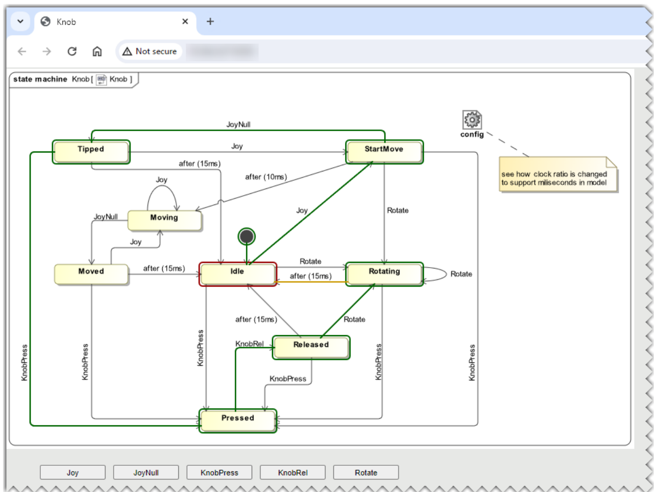
State Machine Diagram simulation on the Web browser.
