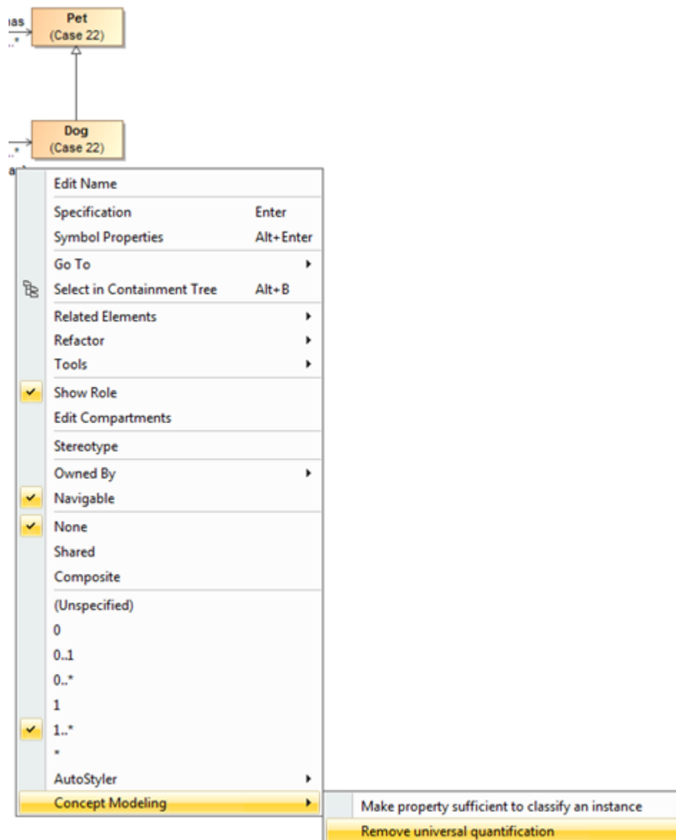
Figure 1: Removing a universal quantification constraint from a property.
