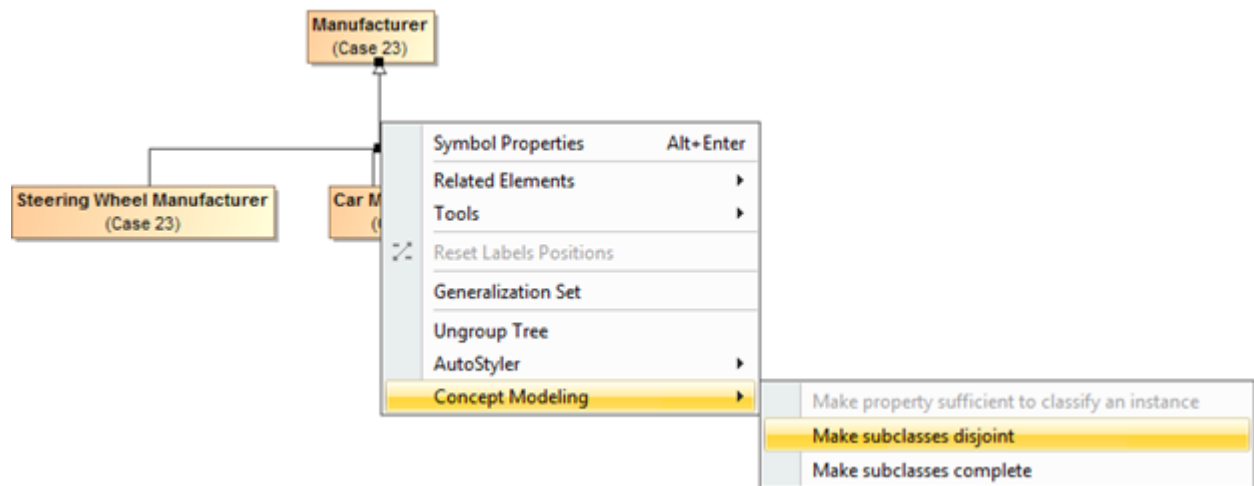
Figure 1: Selecting the Make subclasses disjoint shortcut menu.
