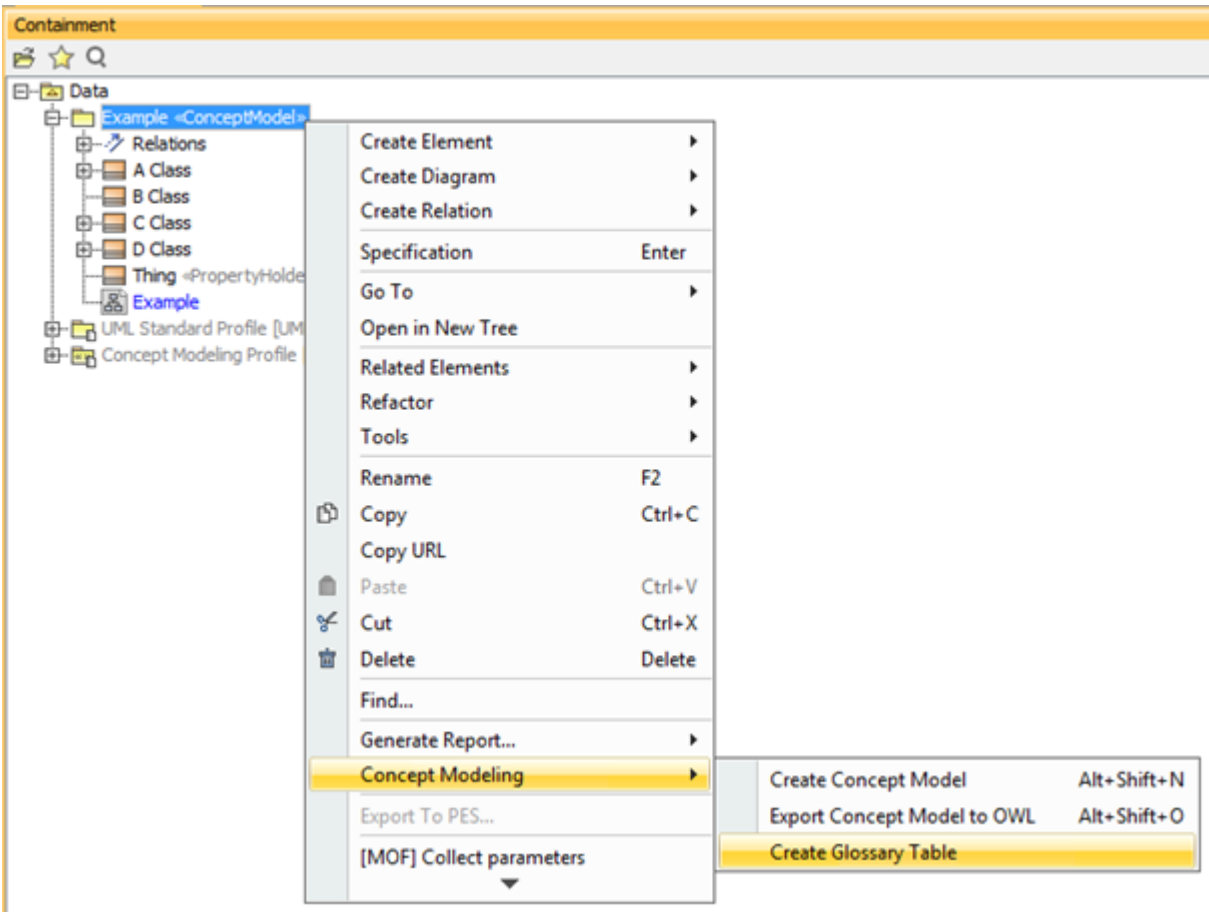
Figure 1: The Concept Modeler's Create Glossary Table menu.
