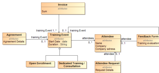
Business Data Diagram showing Classes
