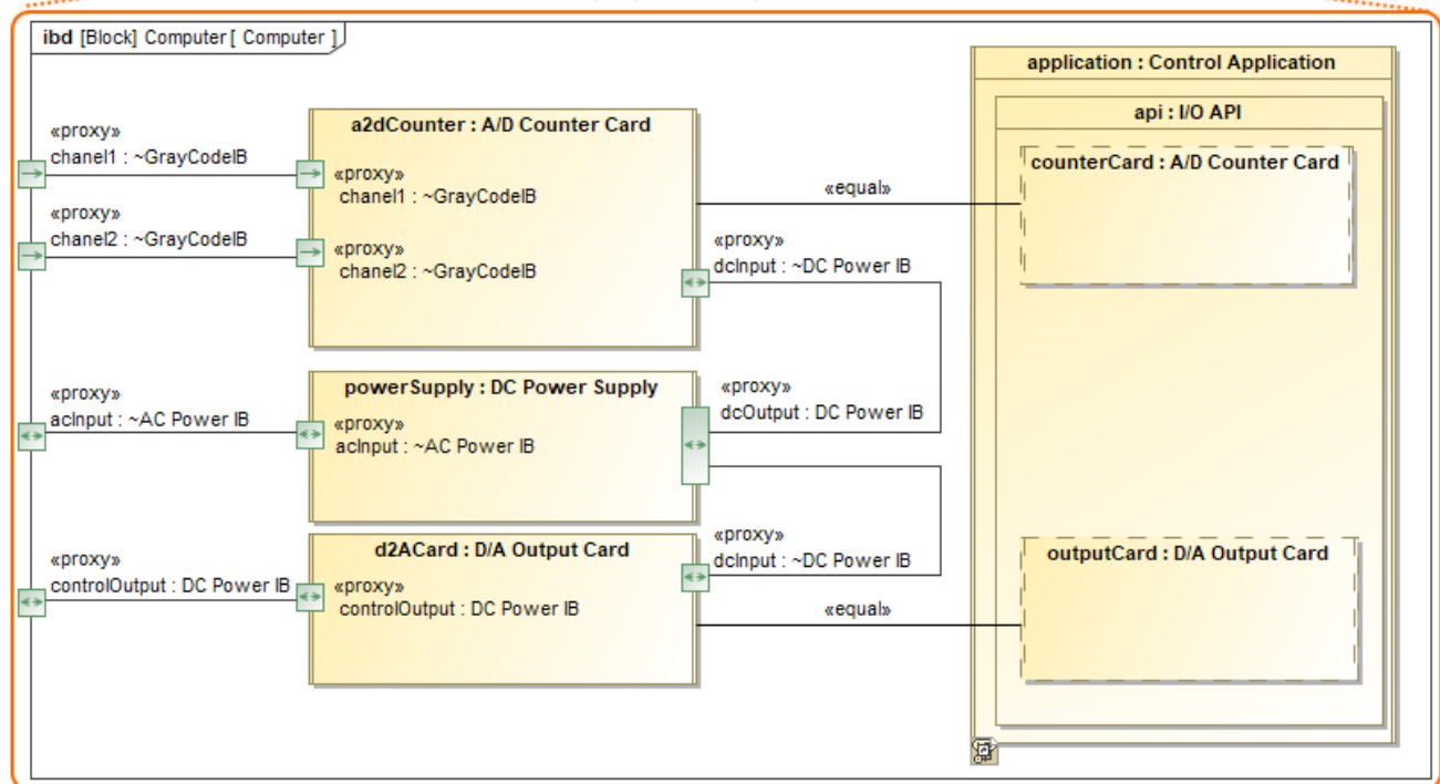
Computer Block properties represented in IBD
