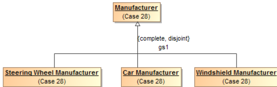
Disjoint and complete subclasses in standard UML notation.
