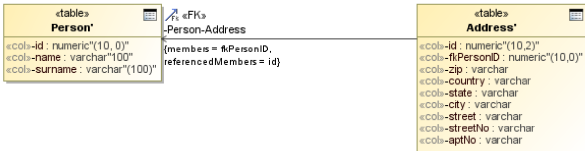
Foreign key example.
