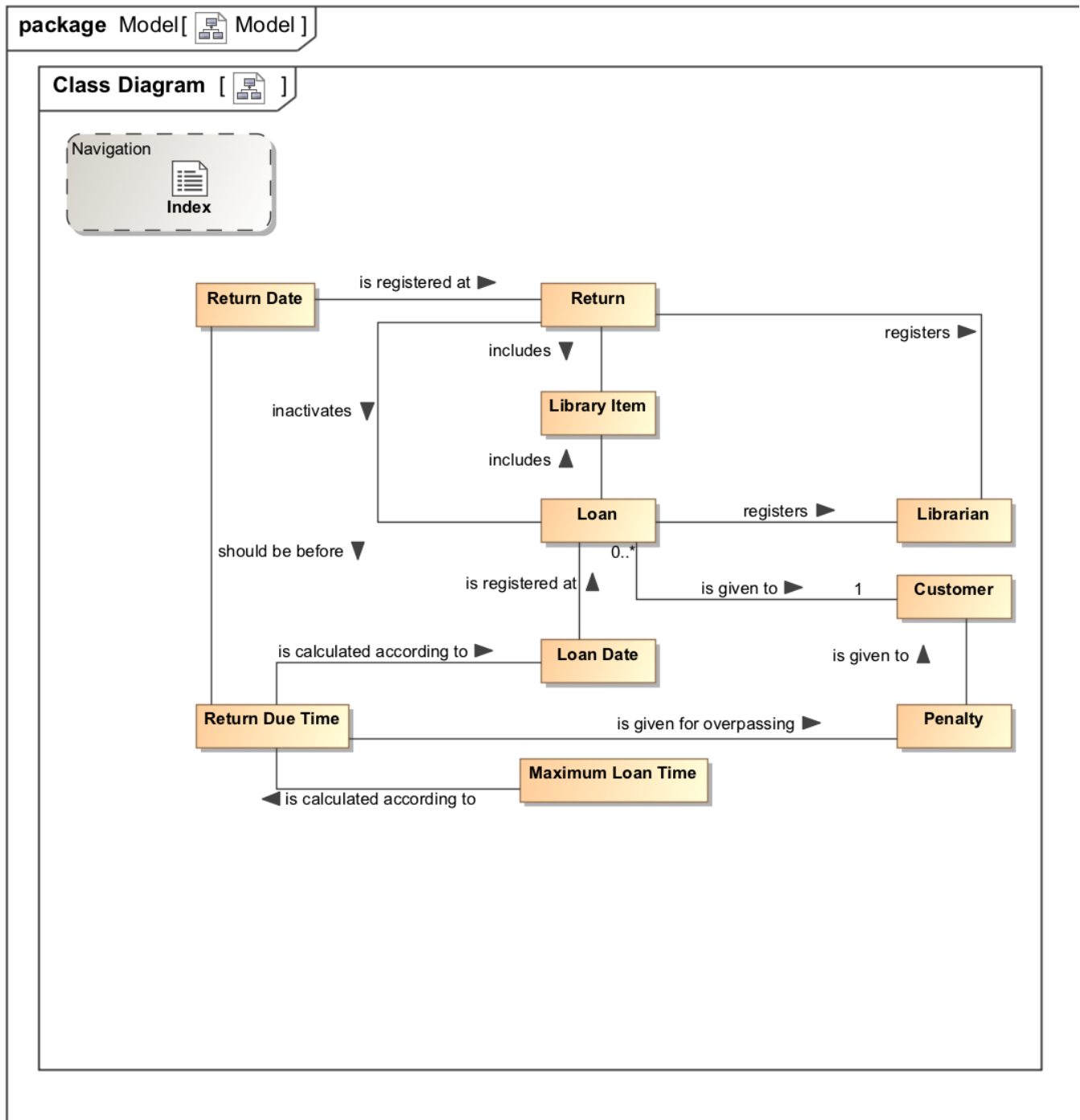
Example of using the Diagram Overview functionality
