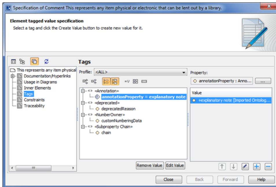
Showing the Annotation Property tagged value of the Annotation in the Specification window.
