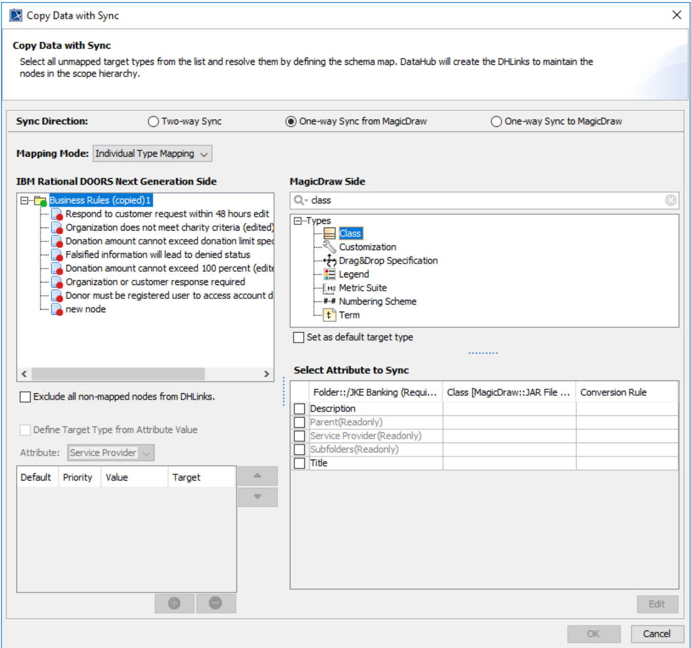
Individual type mapping mode in the Copy Data with Sync dialog.
