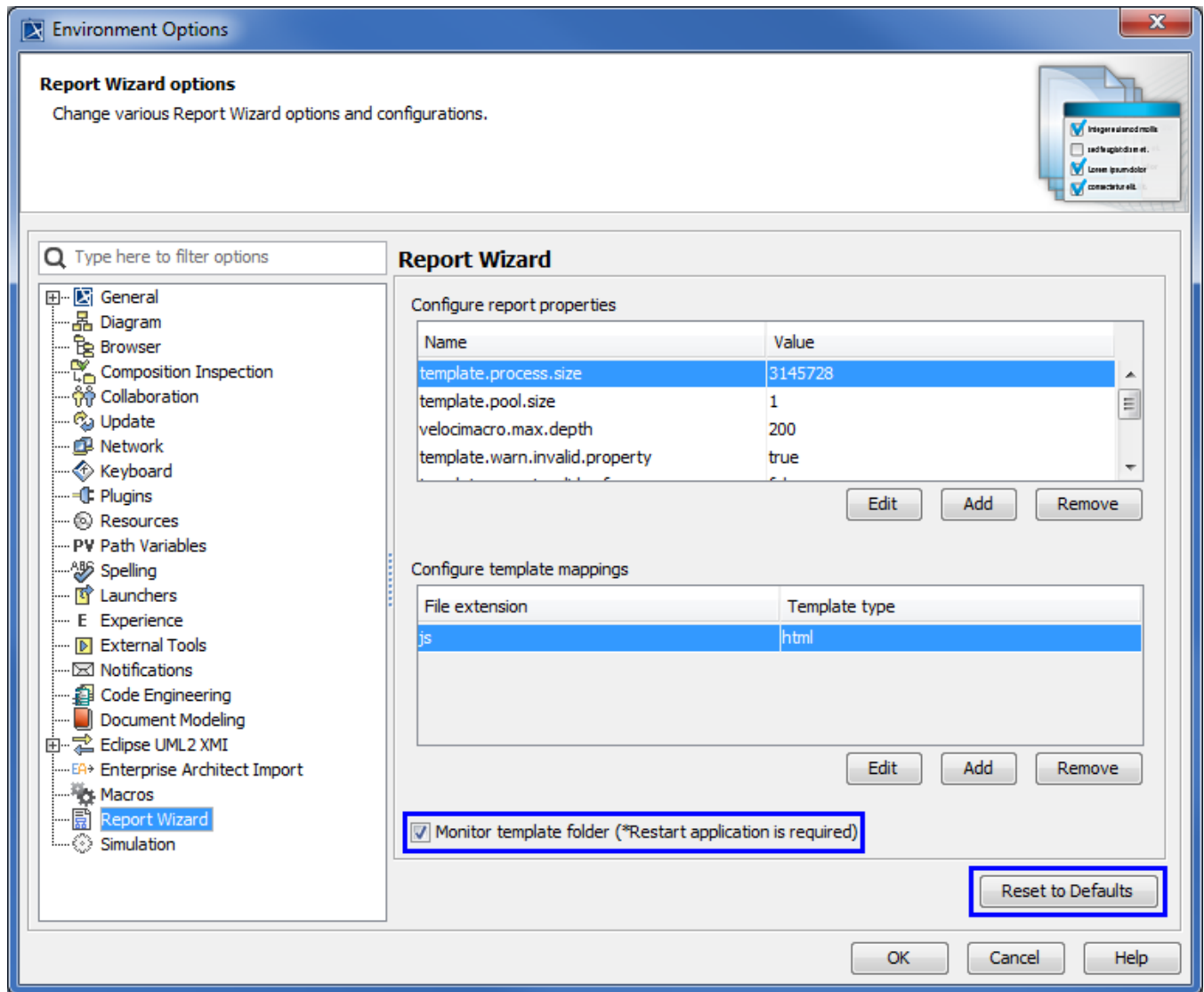
The Monitor template folder and Reset to Defaults options of Report Wizard in the MagicDraw's Environment Options dialog.
