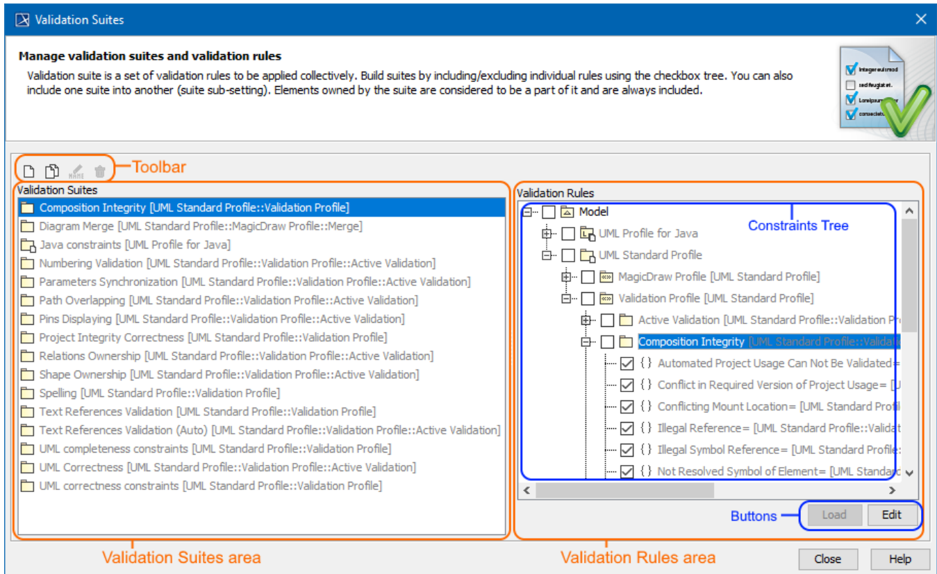
The Validation Suites dialog areas: toolbar, Validation Suites, and Validation Rules areas.
