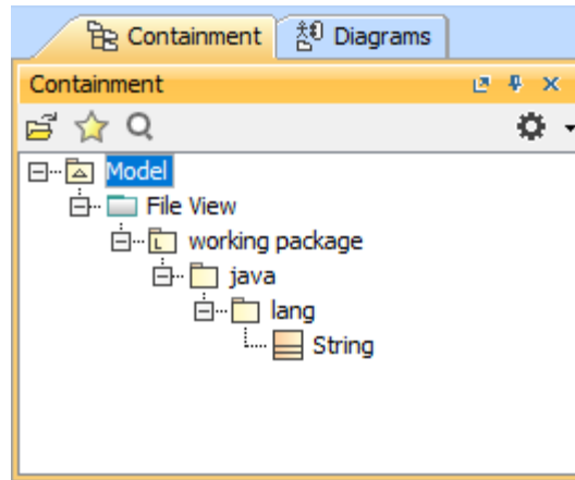
Package Structure
