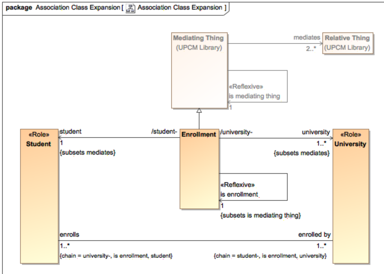
Example of an Expanded UML Association Class Pattern
