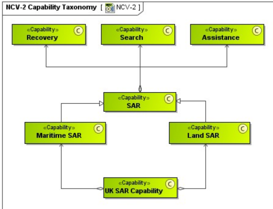
NCV-2 Capability Taxonomy
