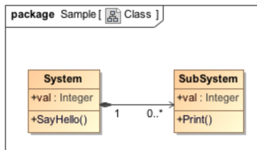
Class diagram describing system Class structure.
