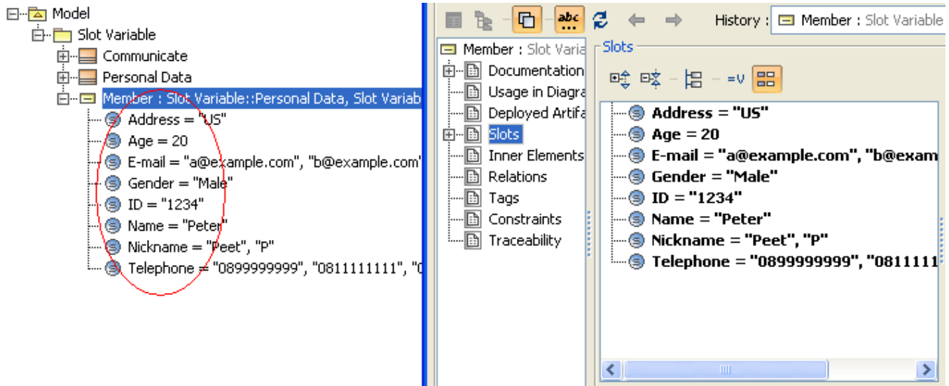
Instance Specification and Slot defining element attributes.
