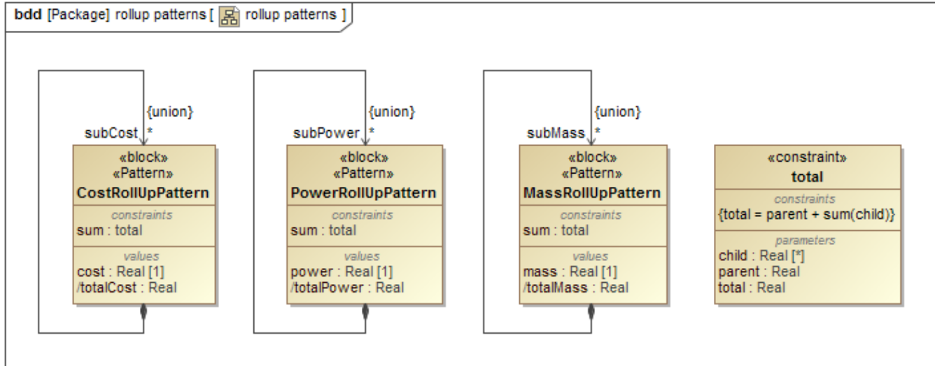
The total cost, mass, or power rollup pattern Blocks defined in the SysML Block Definition Diagram.
