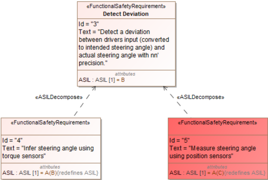
Illustration of the ASIL Decomposition validation rule.
