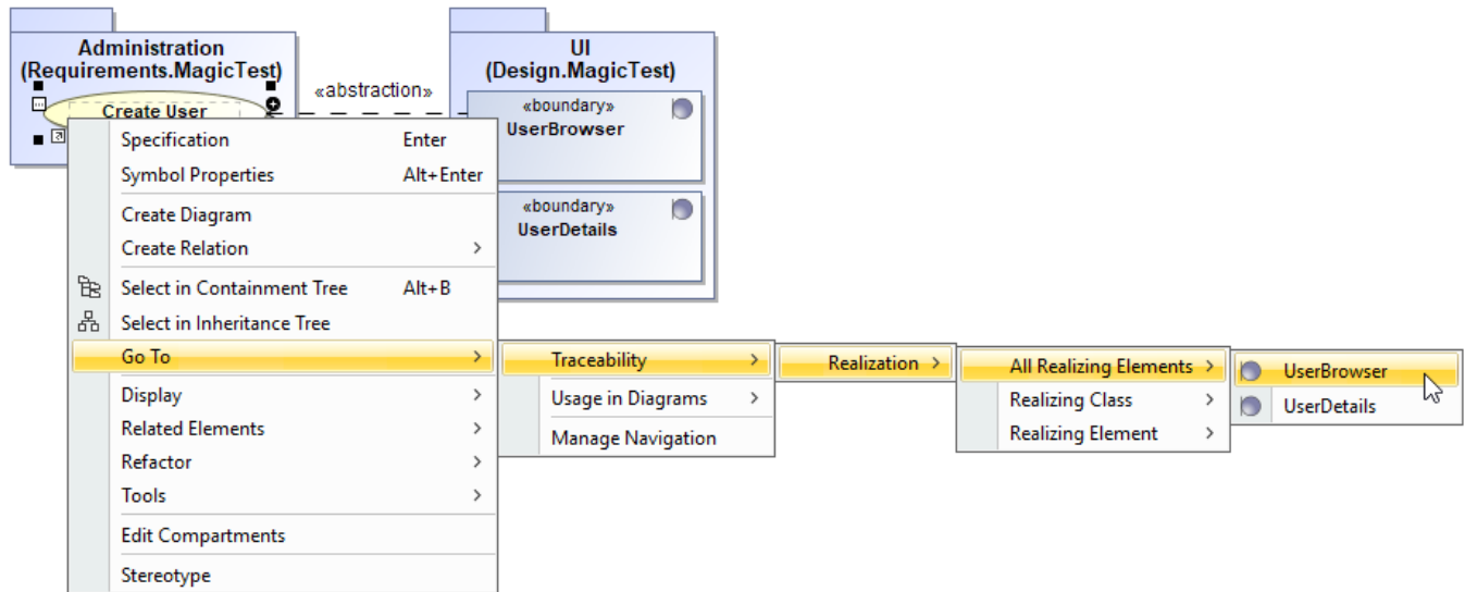
Traceability properties in the Go To submenu
